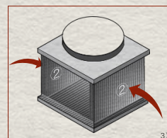
Place the two pieces of carbon filter number ② on the symmetrical sides of the recirculation kit
