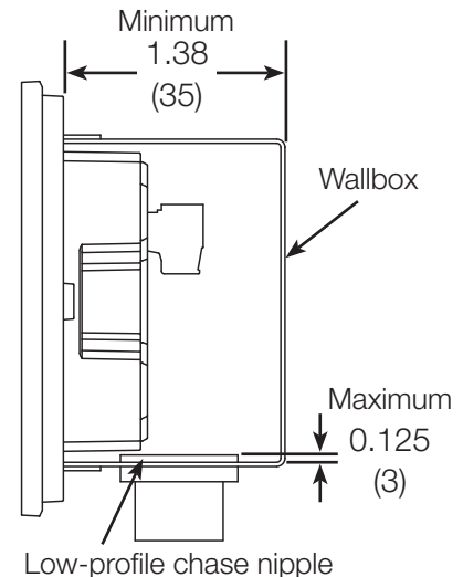
Thermostat, adapter, and metal wallbox
