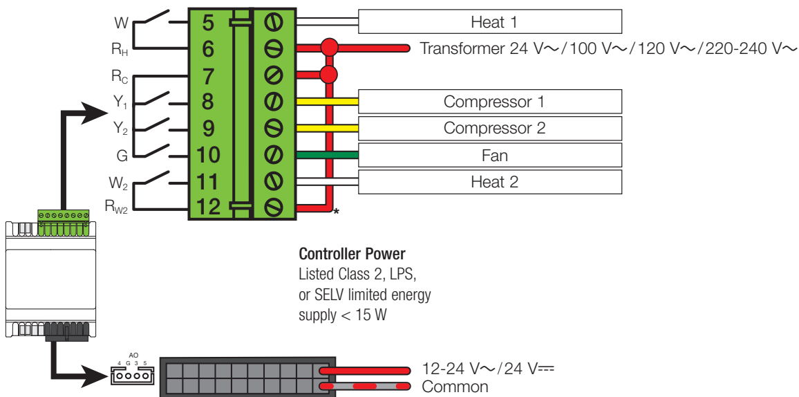
Diagram 10: 2 heat stages/2 cool stages system (1 transformer)
