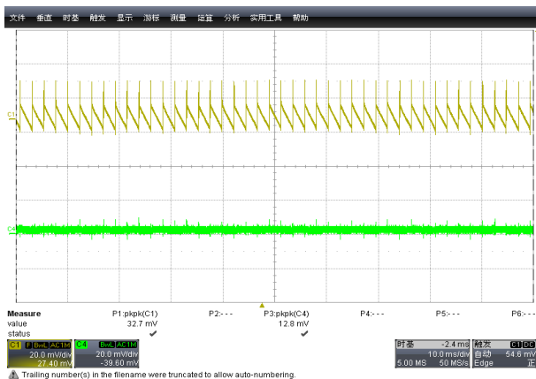
Figure 22: 90Vac/60Hz 9V/3A \Delta V=32.7\text{mV}
