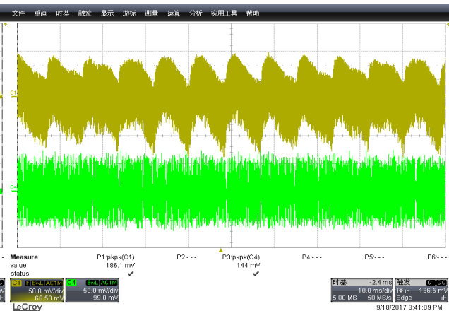
Figure 25: 264Vac / 60Hz 15V/0A \Delta V=186\text{mV}
