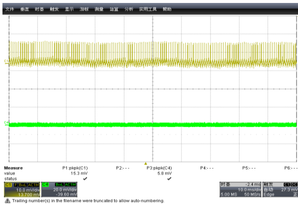
Figure 20: 90Vac/60Hz 9V/0A \Delta V=15.3\text{mV}
