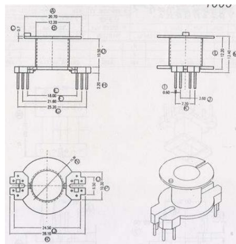
Figure 5: RM10 Bobbin & Pin assignments
