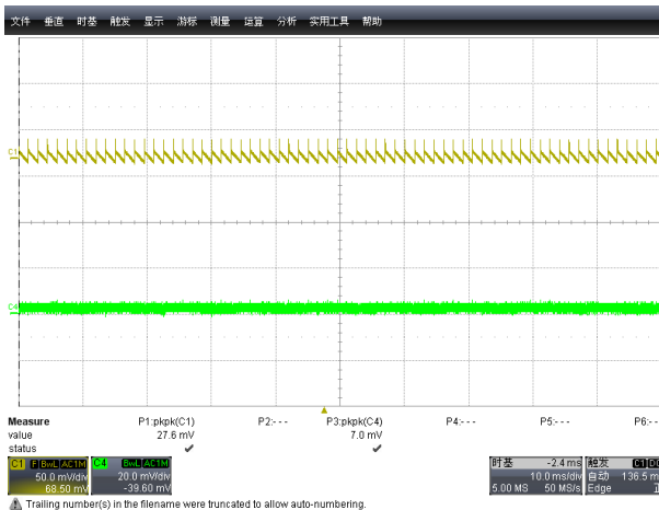
Figure 16: The Ripple at 90Vac/60Hz \Delta V=30\text{mV} 5V/0A
