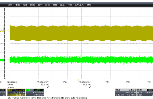
Figure 19: 264Vac/50Hz 5V/3A \Delta V=90\text{mv}
