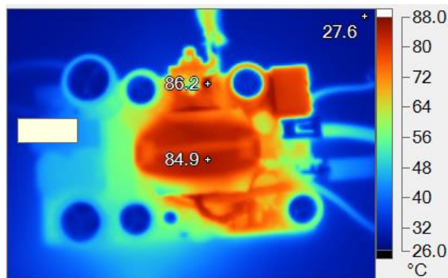
Figure 45: Top components side
