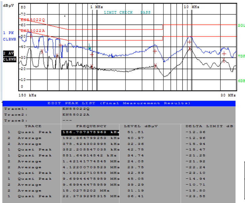
Figure 47: 115Vac/60Hz 15V/3A (N)
