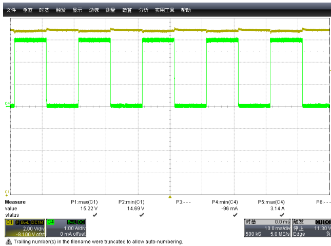
Figure 34: 90Vac / 60Hz 15V/ 0~3A \Delta V=53mV
