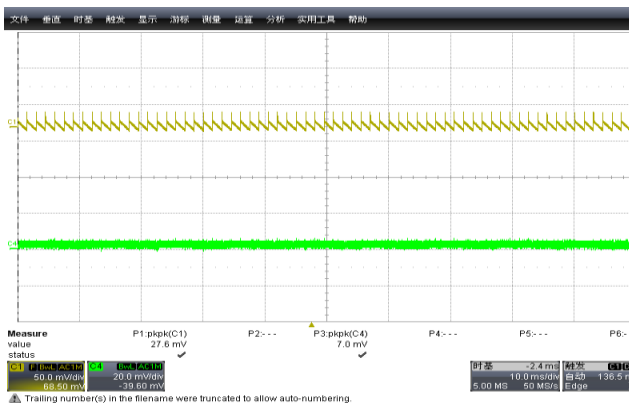
Figure 18: 90Vac/60Hz 5V/3A \Delta V=68.5\text{mV}
