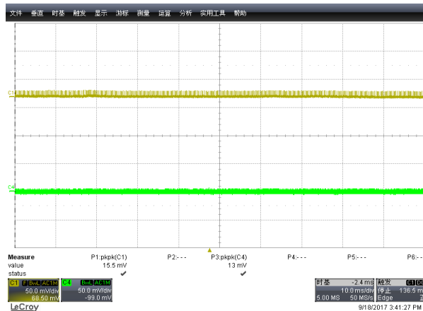
Figure 24: 90Vac/60Hz 15V/0A \Delta V=15.5\text{mV}
