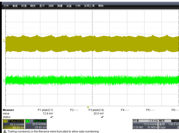
Figure 17: The Ripple at 264Vac/50Hz \Delta V=72.8\text{mv} 5V/0A
