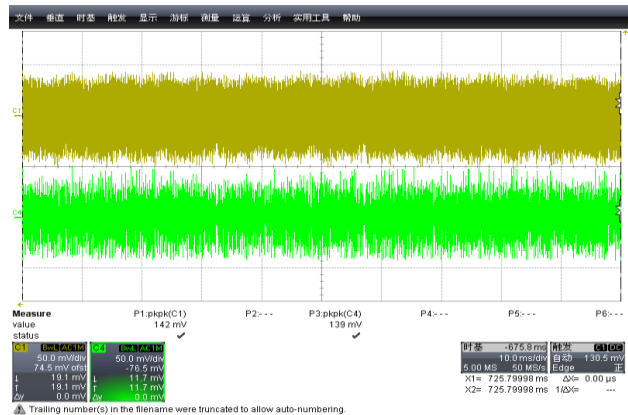
Figure 21: 264Vac/50Hz 9V/0A \Delta V=142\text{mV}
