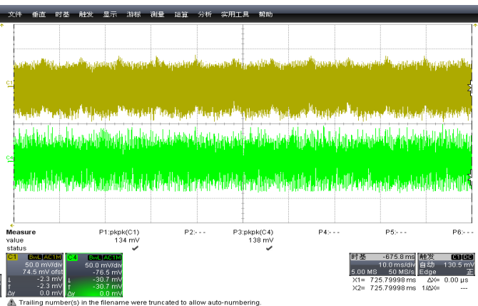
Figure 23: 264Vac / 60Hz 9V/3A \Delta V=134\text{mV}
