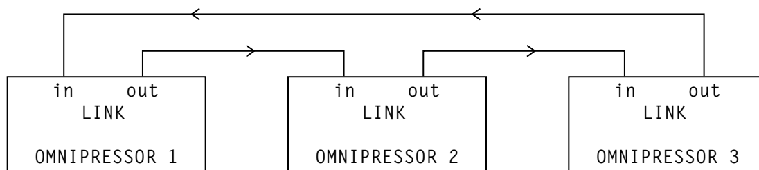
MULTI-UNIT LINKING---BLOCK DIAGRAM
