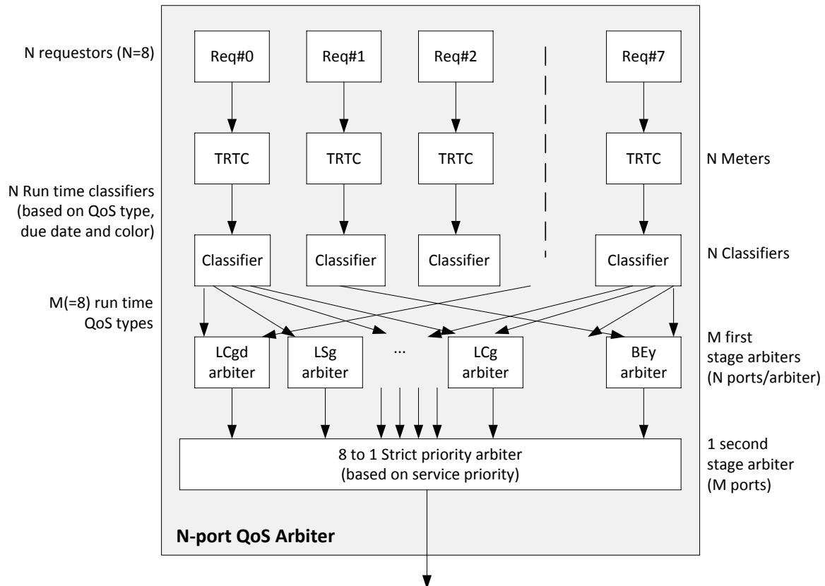
Figure 5-3 QoS Arbitration Block Diagram
