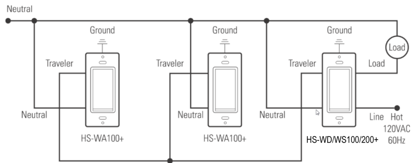
4-way circuit
