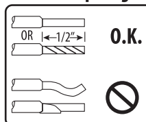
Wires/Strip Length
