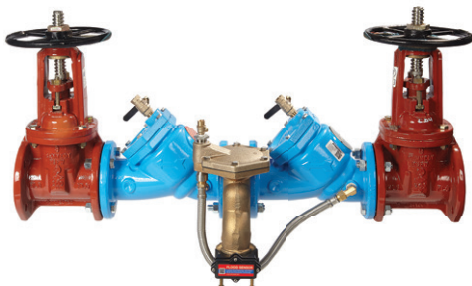
LF909 with flood sensor
