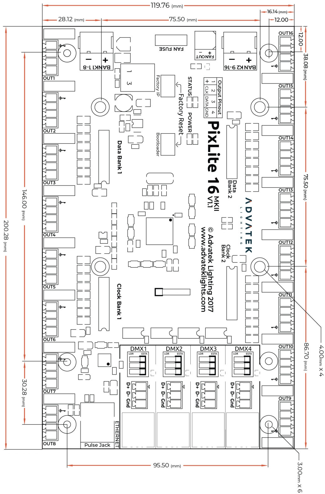
Figure 13: Mechanical Specifications
