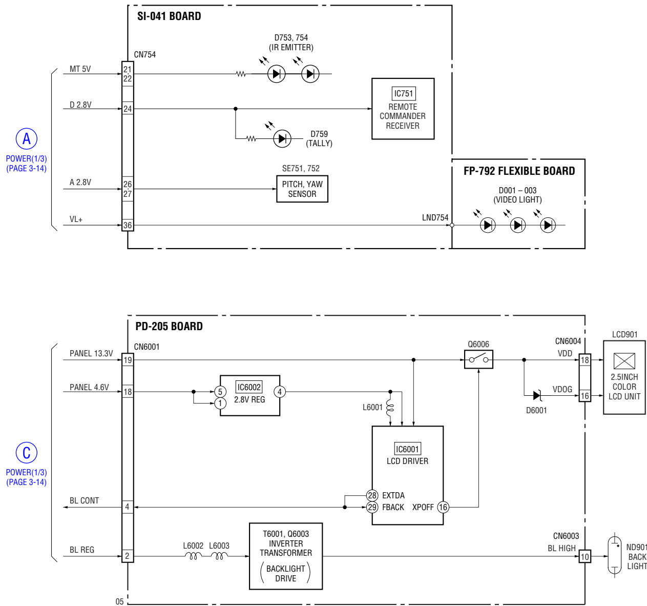
3-9. POWER BLOCK DIAGRAM (3/3) ( ) : Number in parenthesis ( ) indicates the division number of schematic diagram where the component is located.
