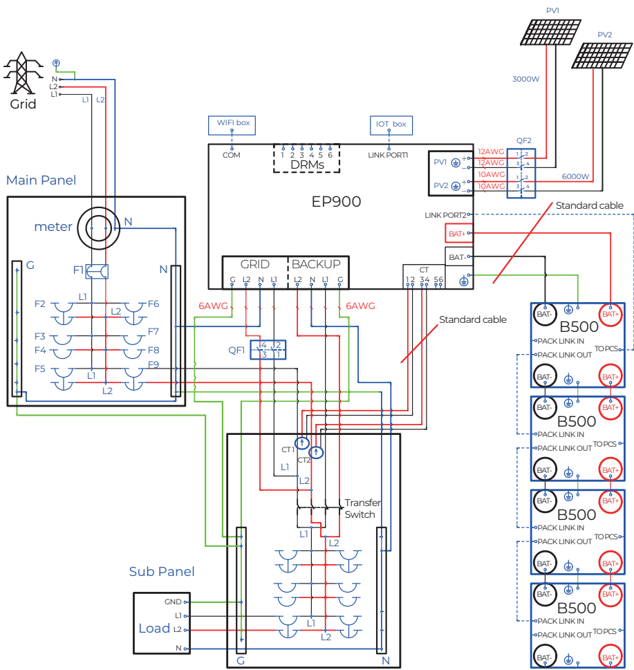
Fig. 7-10 Partial backup system
