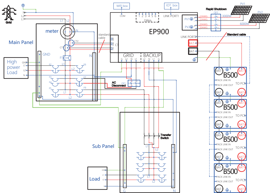
Fig. 7-11 Self-Consumption and Partial backup system
