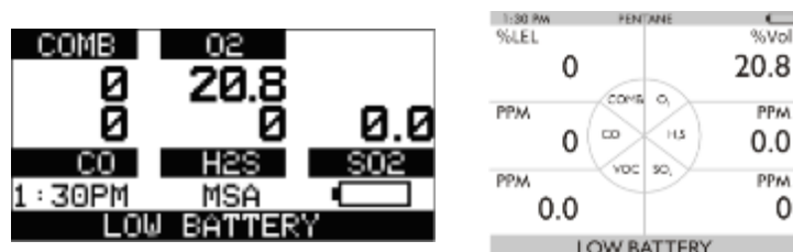
Figure 4 Battery Warning
