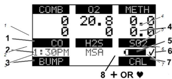
Figure 2 Monochrome Display
