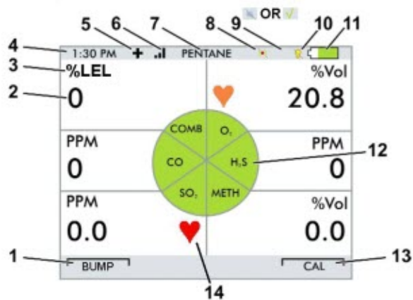
Figure 3 Color display
