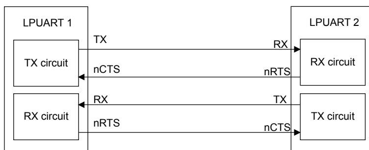
Figure 147. Hardware flow control between 2 LPUARTs
