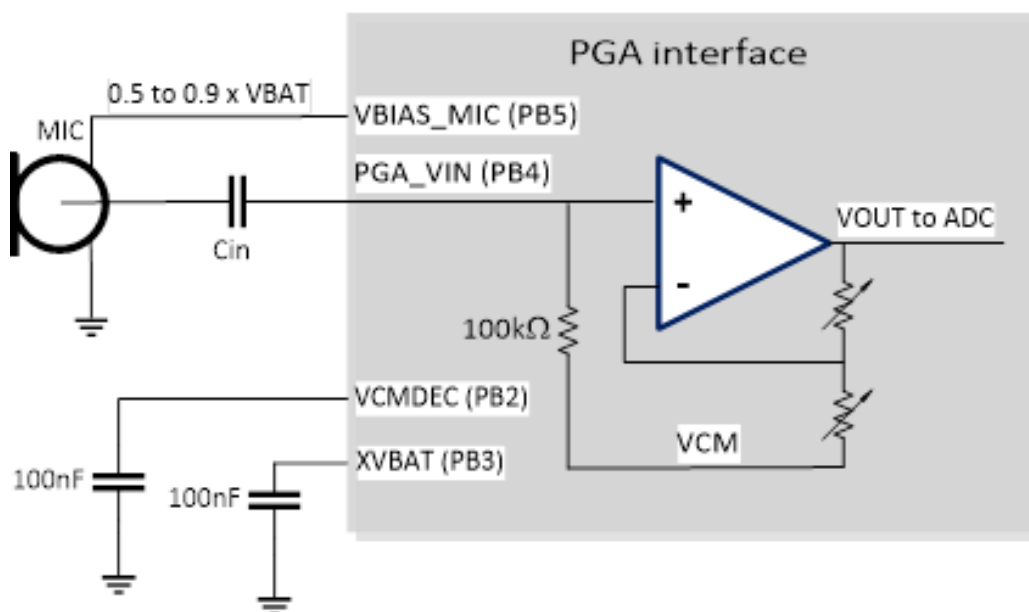
Figure 23. Microphone setup
