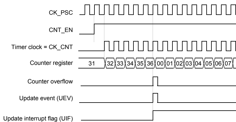
Figure 32. Counter timing diagram, internal clock divided by 2
