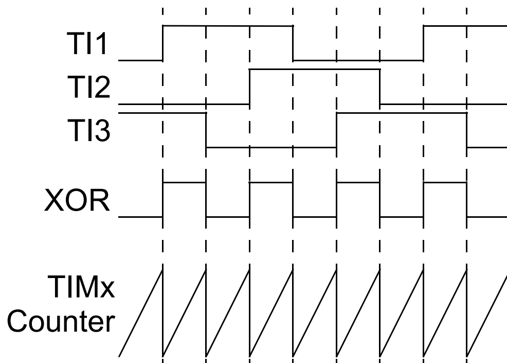
Figure 80. Measuring time interval between edges on 3 signals
