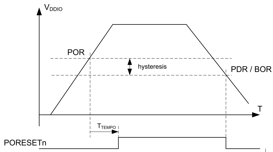
Figure 5. Power-on reset/power-down reset waveform
