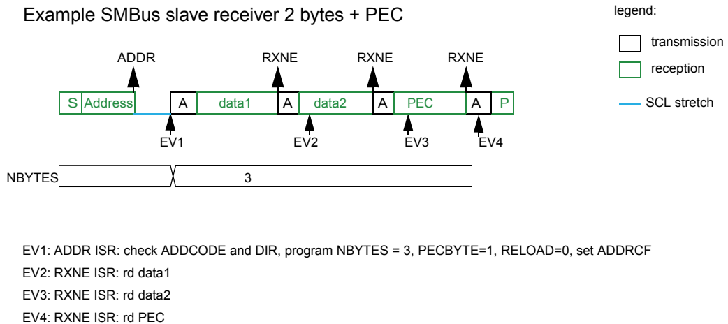
Figure 109. Bus transfer diagrams for SMBus slave receiver (SBC=1)
