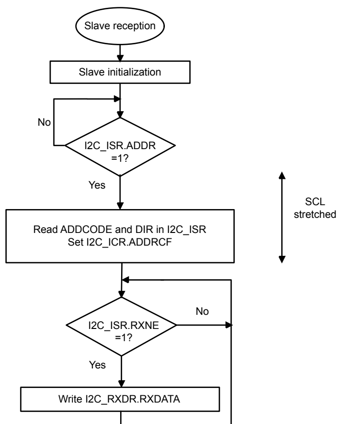
Figure 93. Transfer sequence flowchart for slave receiver with NOSTRETCH=0
