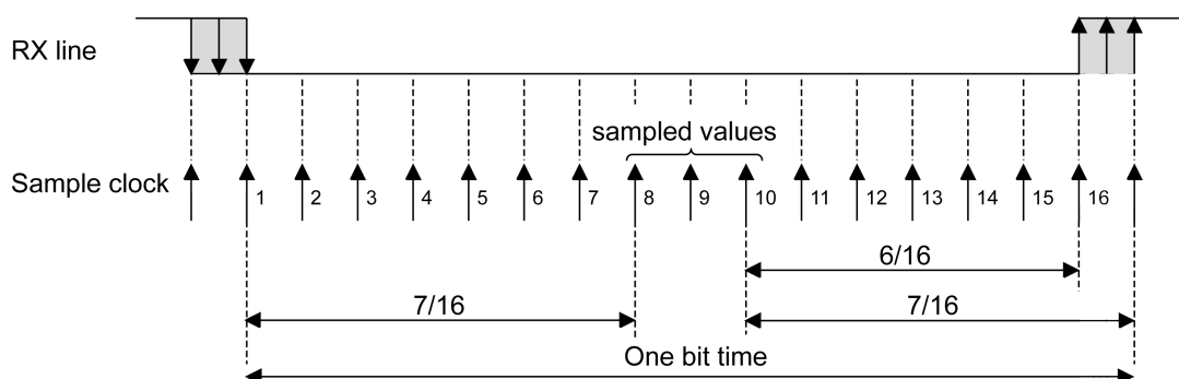
Figure 119. Data sampling when oversampling by 16
