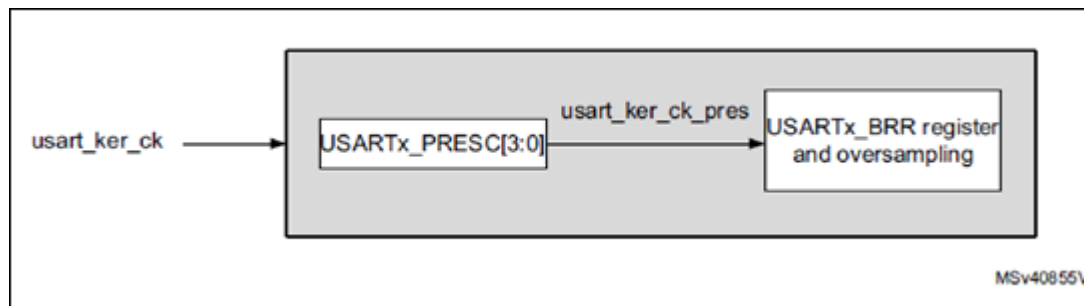
Figure 118. usart_ker_ck clock divider block diagram
