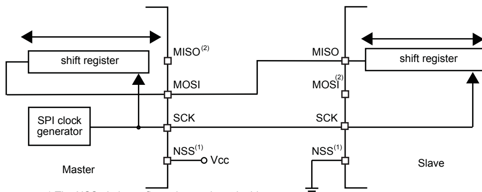
Figure 152. Half-duplex single master/single slave application
