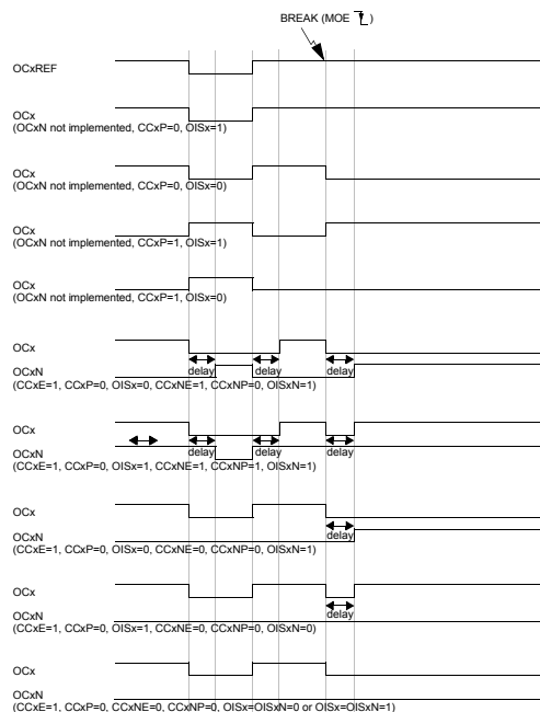
Figure 71. Various output behavior in response to a break event on BRK (OSSI = 1)
