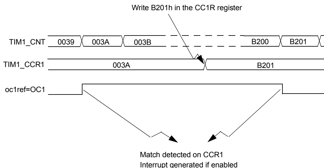
Figure 61. Output compare mode, toggle on OC1
