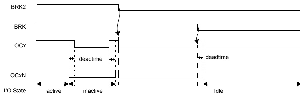
Figure 73. PWM output state following BRK assertion ( OSSI=0 )
