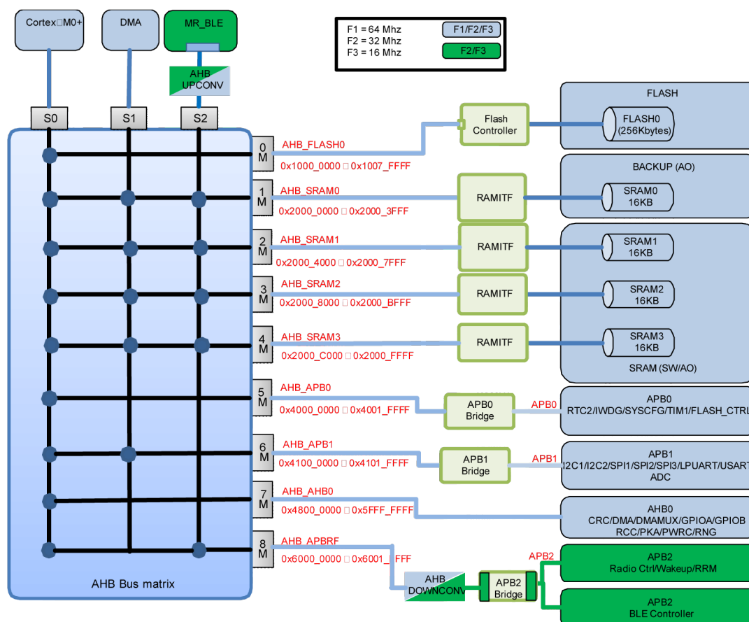
Figure 1. BlueNRG-LP system architecture
