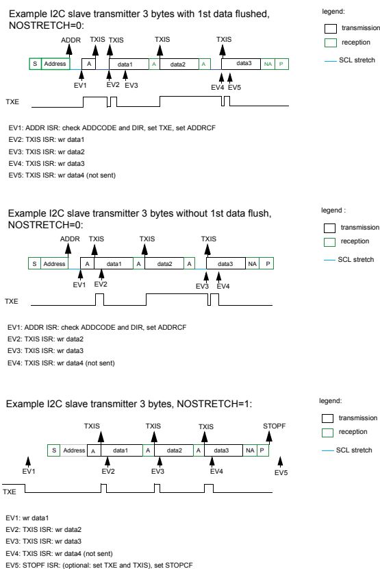
Figure 92. Transfer bus diagram for I2C slave transmitter
