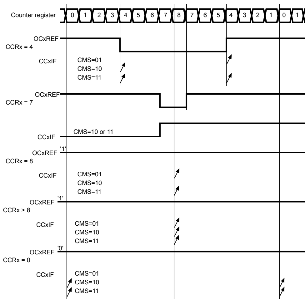
Figure 63. Center-aligned PWM waveforms (ARR=8)
