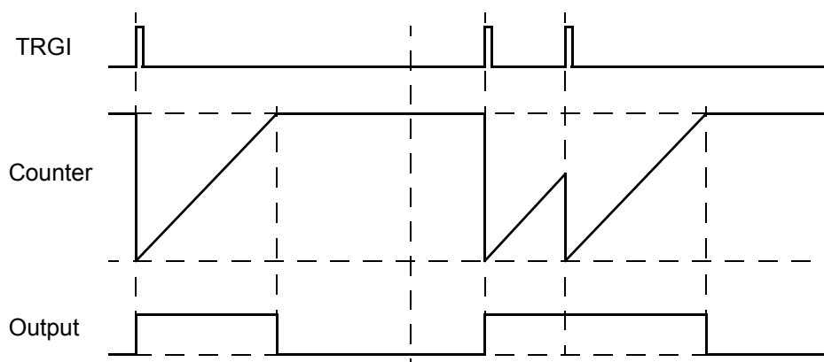
Figure 77. Retriggerable one-pulse mode
