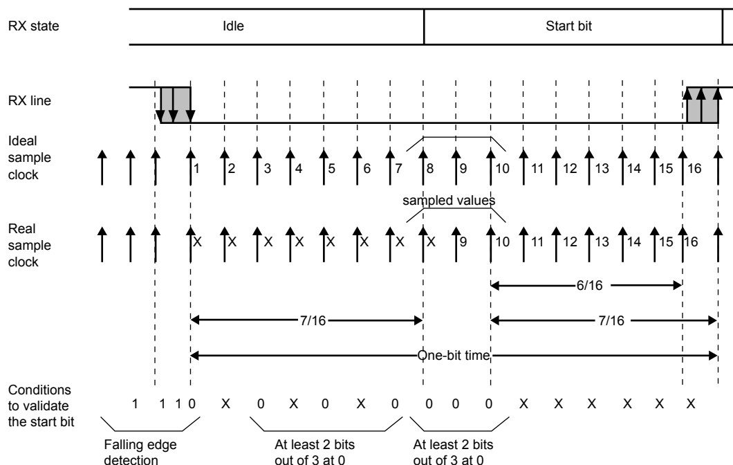
Figure 117. Start bit detection when oversampling by 16 or 8
