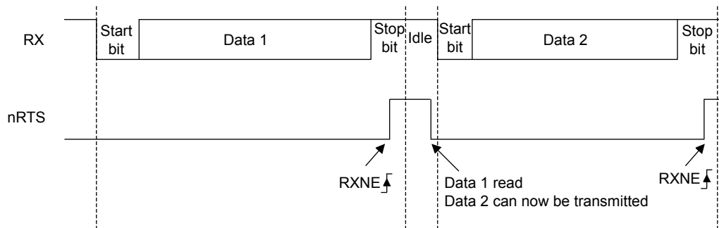
Figure 148. RS232 RTS flow control
