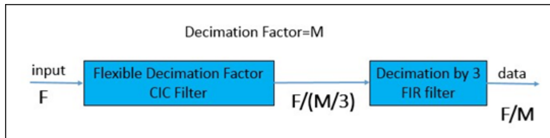
Figure 26. Simplified decimation filter block diagram
