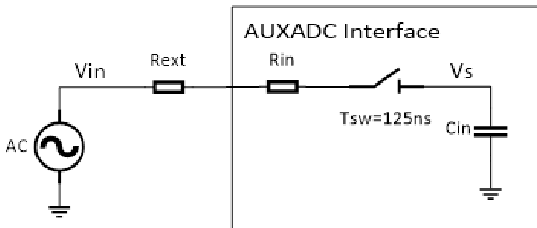
Figure 25. Effect of analog source resistance
