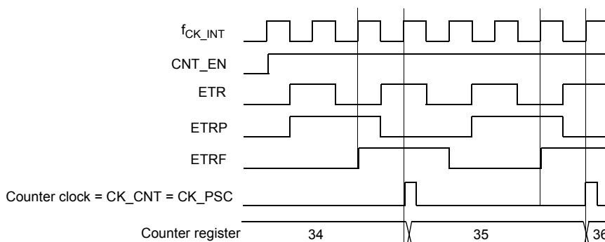
Figure 54. Control circuit in external clock mode 2
