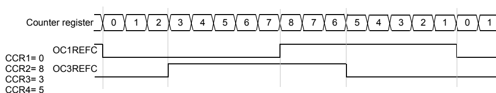
Figure 64. Generation of 2 phase-shifted PWM signals with 50% duty cycle
