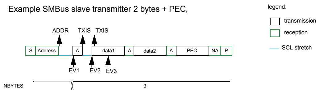
Figure 107. Transfer bus diagrams for SMBus slave transmitter (SBC=1)
