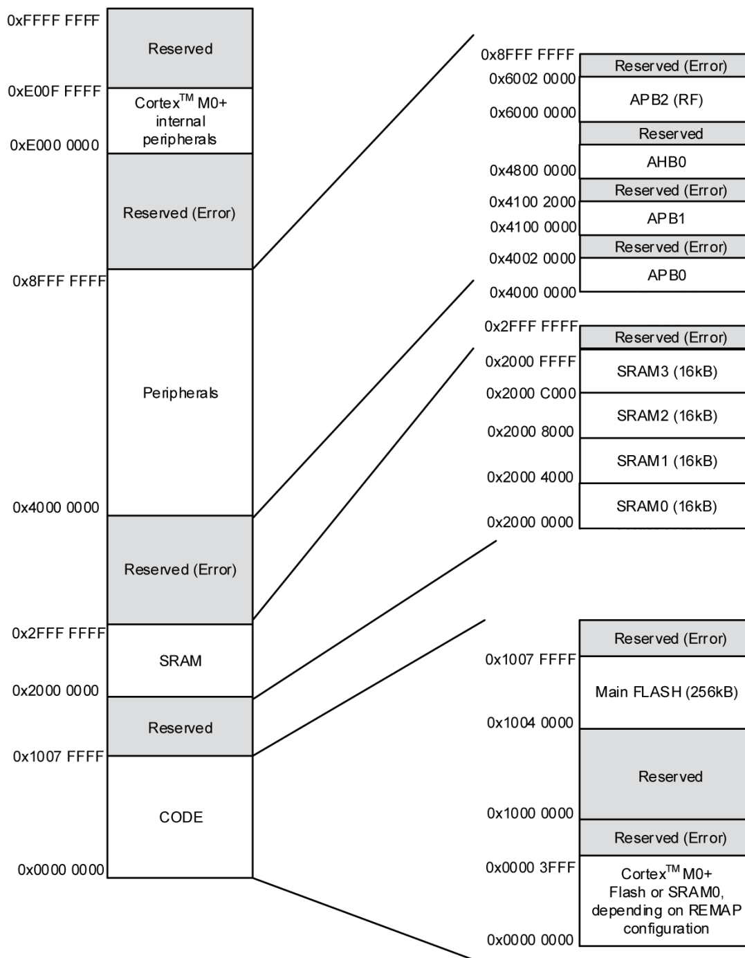
Figure 2. Memory map
