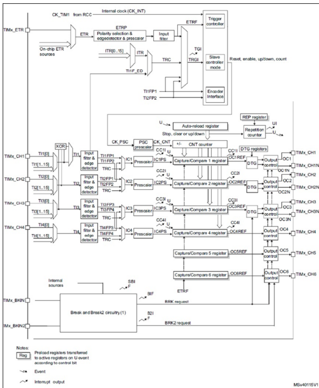
Figure 28. Advanced-control timer block diagram
