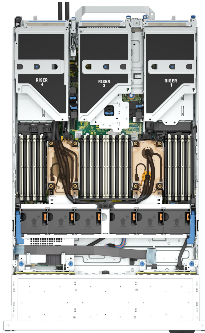
Figure 13. Inside the system with processor liquid cooling module
