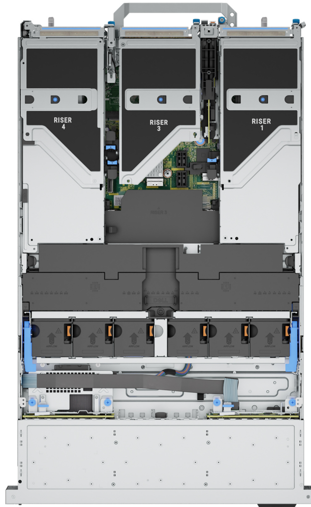
Figure 12. Inside the system with full length risers and GPU shroud
