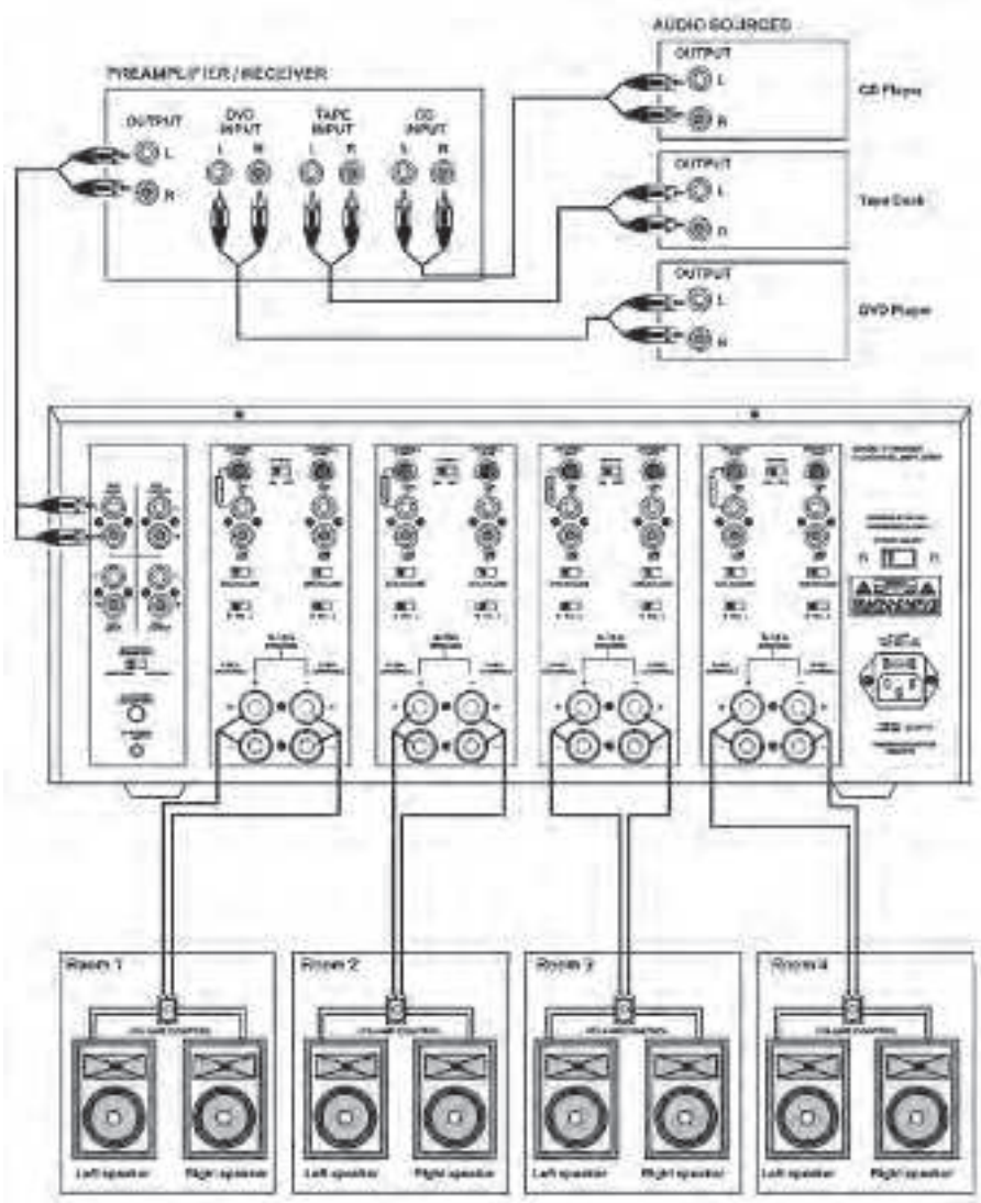
DIAGRAM 4 - MULTI-ROOM INSTALLATION
