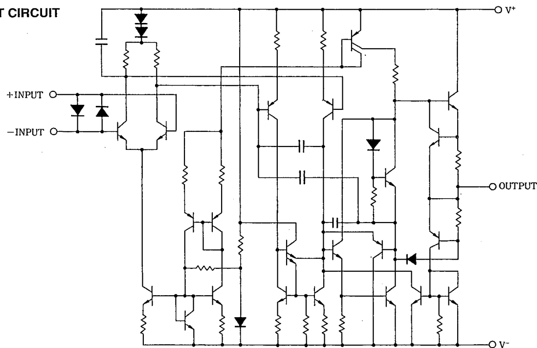
NJM5532D NJM5532M
