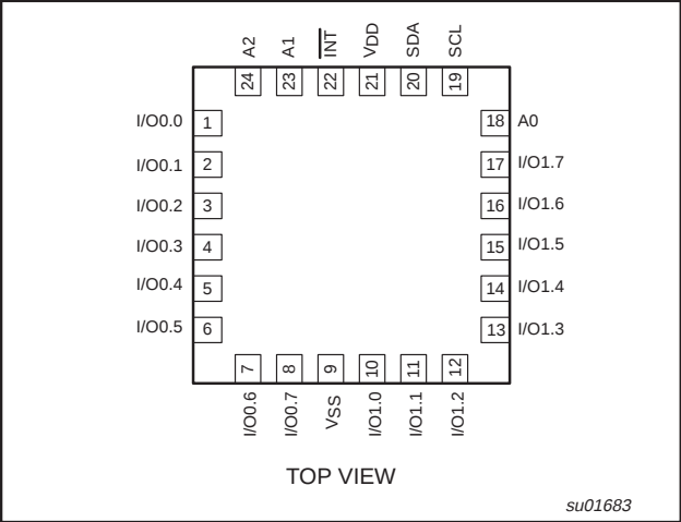
Figure 2. Pin configuration — HVQFN
