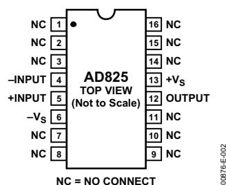
Figure 2. 16-Lead Plastic SOIC (R-16) Package
