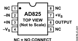
Figure 1. 8-Lead Plastic SOIC (R) Package
