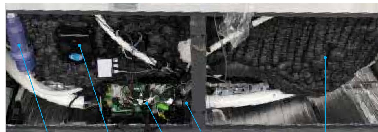
Ozone Mixing Chamber Ozone Generator Control pack Heater Black out insulation
