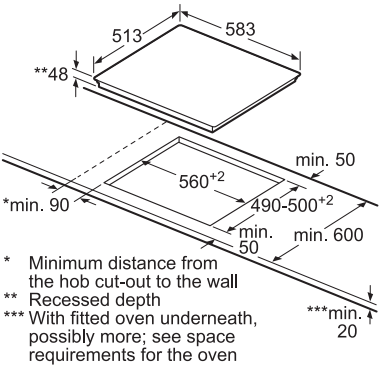
quickLite ceramic hob ET645CEA1E
