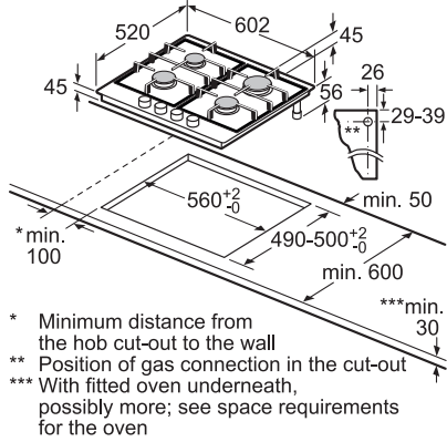
Gas hob ER6A6PD70
