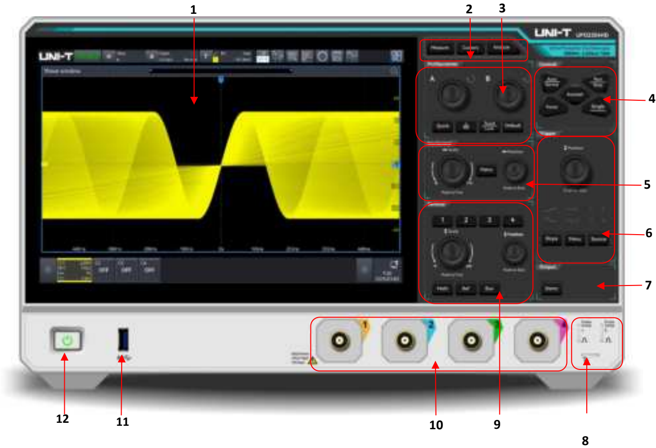
Front Panel
