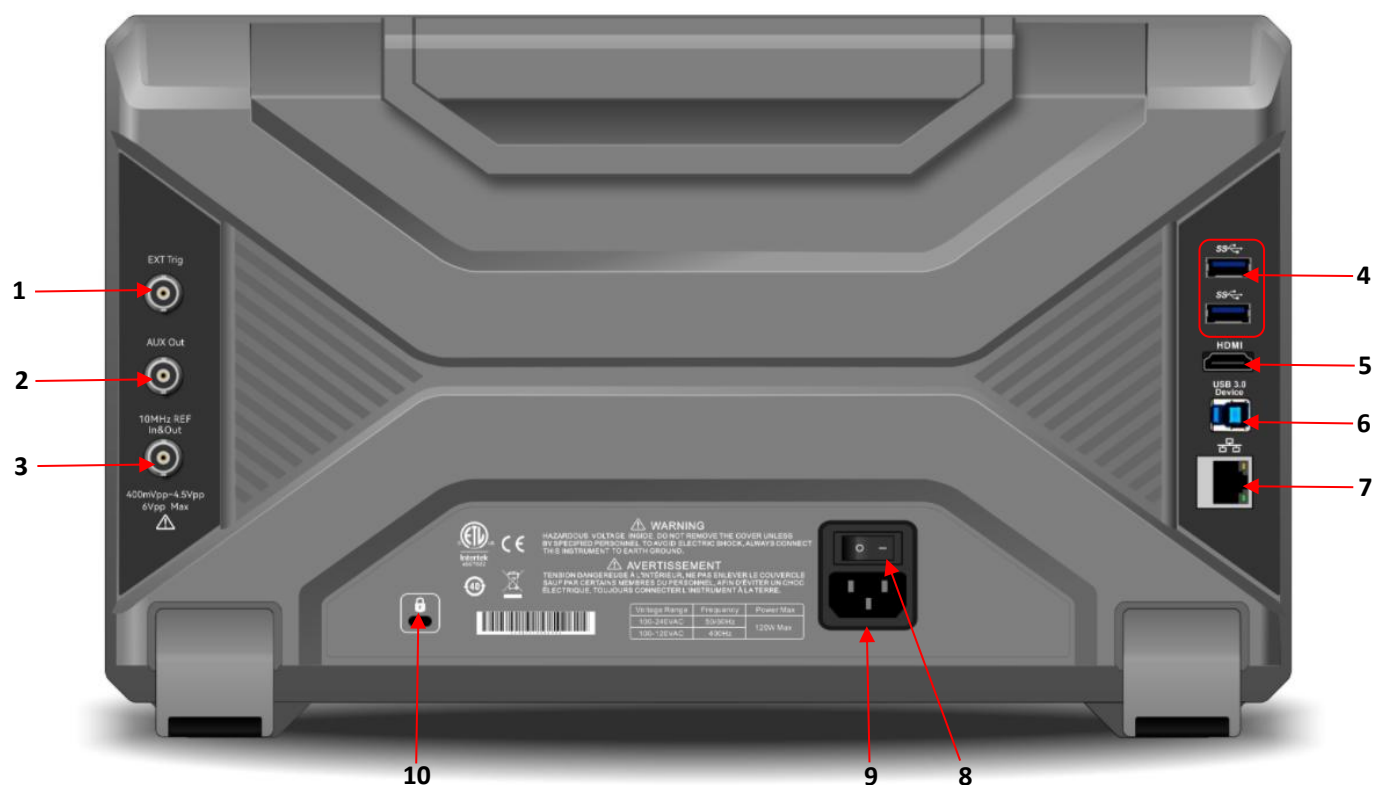
Rear Panel
