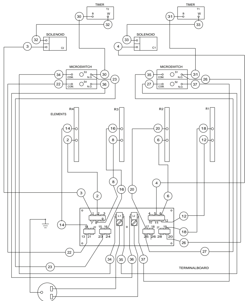
TERMINAL BOARD WIRING 120V
