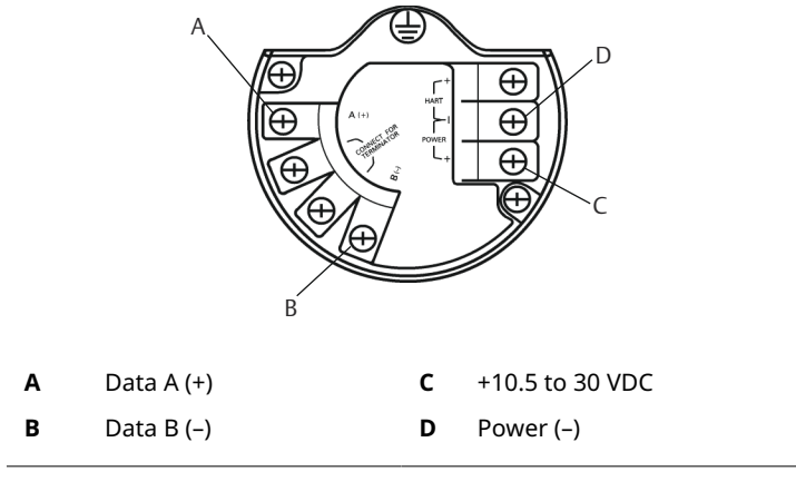
Figure 2-2: Emerson Wireless Field Link Terminal Diagram
