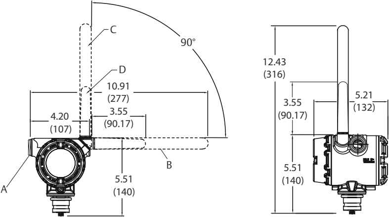
Figure 4-2: Emerson Wireless Field Link Dimensional Drawing
