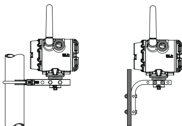
Figure 2-1: Mounting
