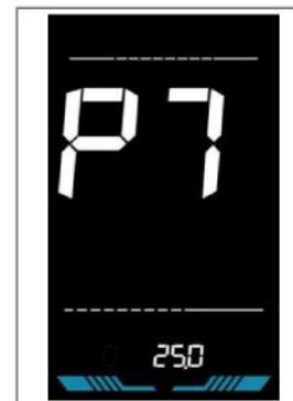
Controller current limit setting interface
