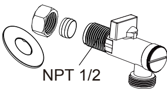
Angle Valve
