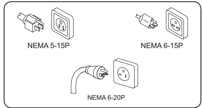
Plug Configurations
