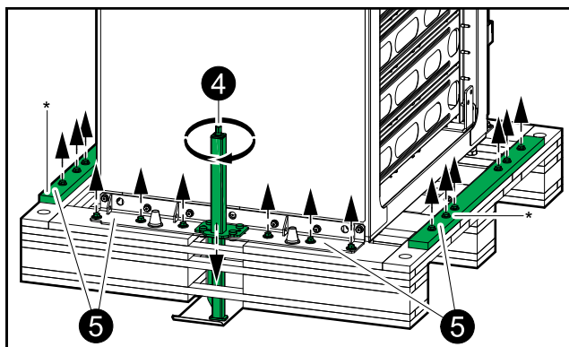
Rear View of the Wide Cabinet
