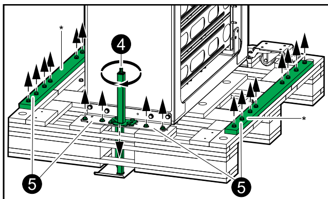
Rear View of the Narrow Cabinet
