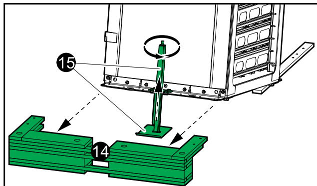
Front View of the Wide Cabinet
