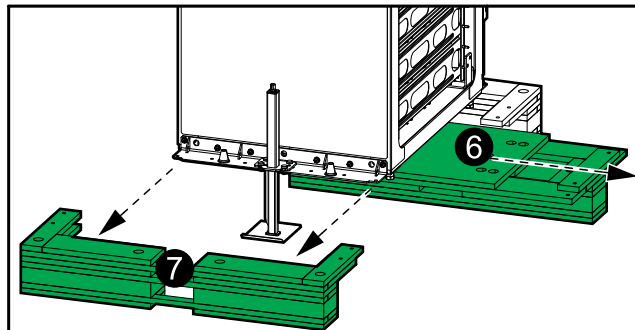
Rear View of the Wide Cabinet
