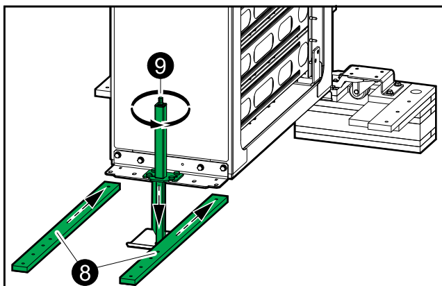
Rear View of the Narrow Cabinet
