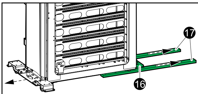
Side View of the Narrow Cabinet
