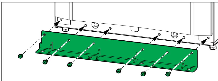
Front View of the Modular Battery Cabinet
