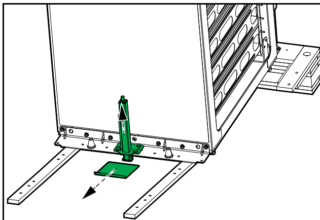
Rear View of the Wide Cabinet
