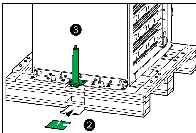
Rear View of the Wide Cabinet
