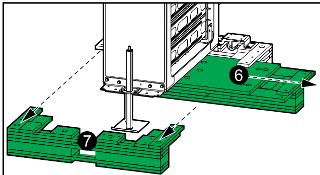
Rear View of the Narrow Cabinet
