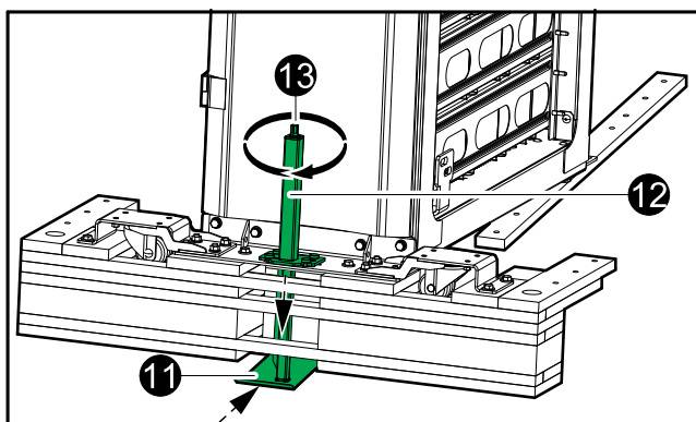
Front View of the Narrow Cabinet
