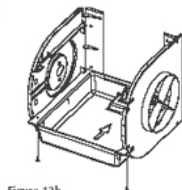
Figure 13b INSTALLING THE FLOAT AND VALVE ASSEMBLY
