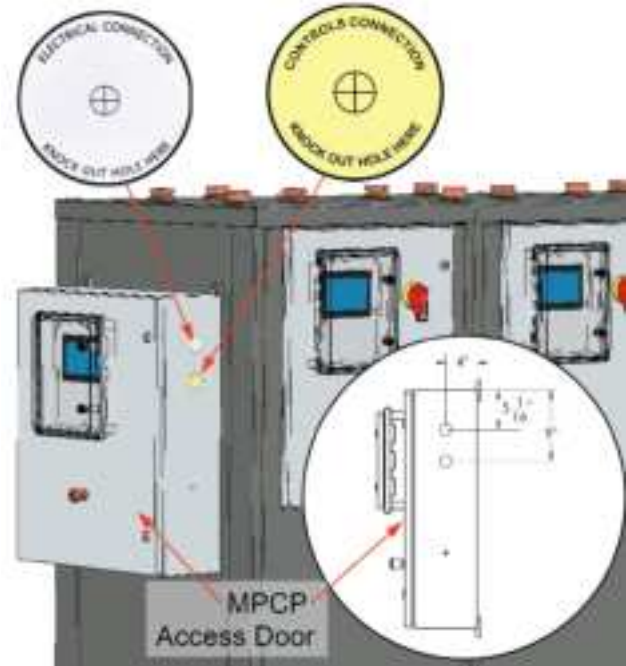
Figure 15. Power wire connections
