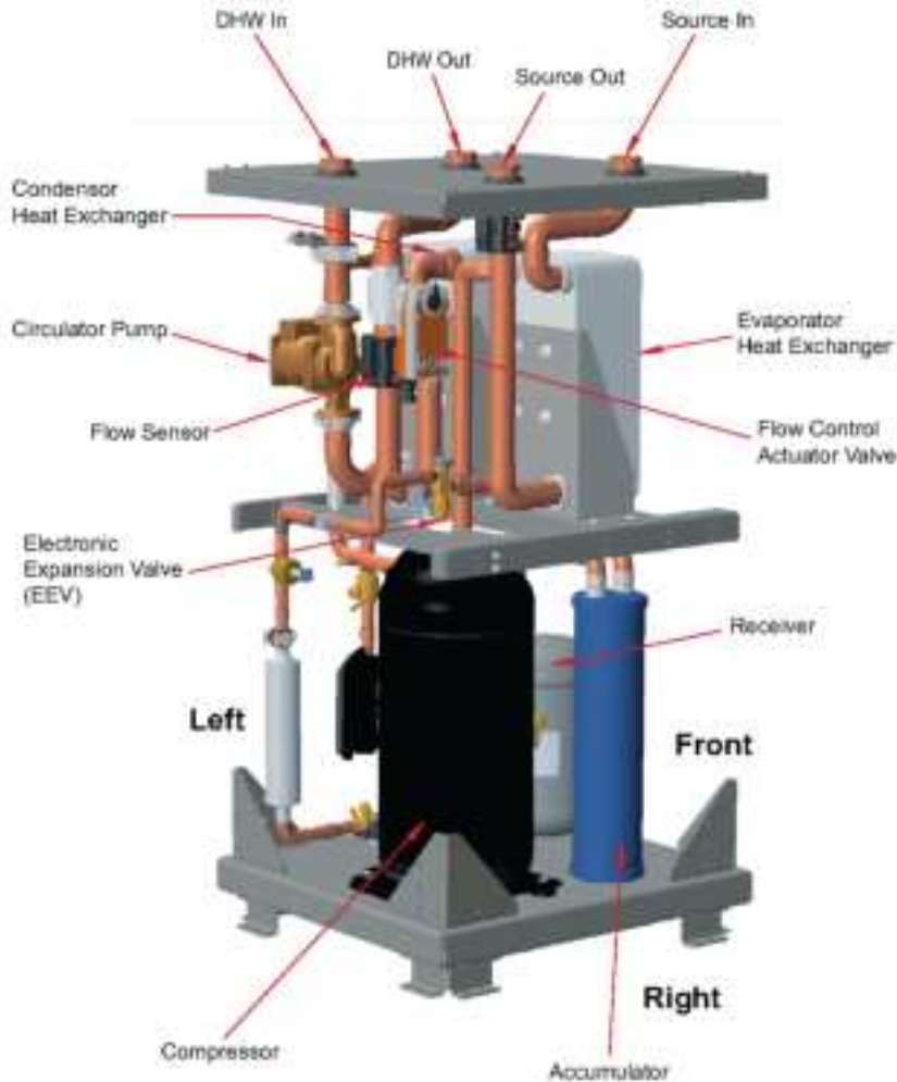
Figure 6. Individual module
