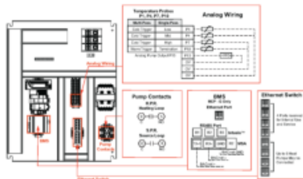
Figure 17. MPCP field wiring connections
