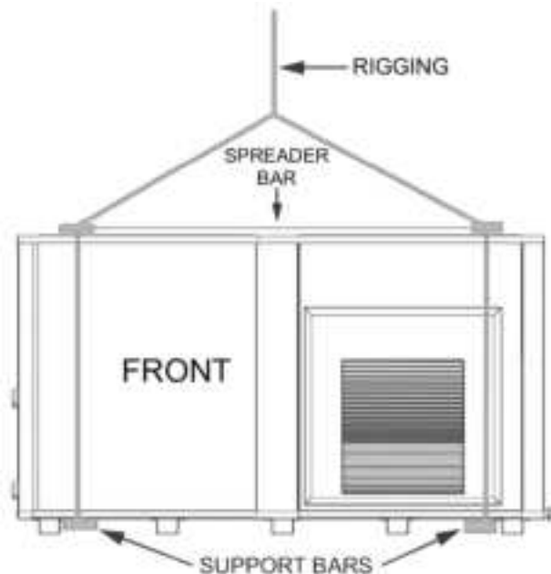
Figure 8. Rigging and hoisting unit
