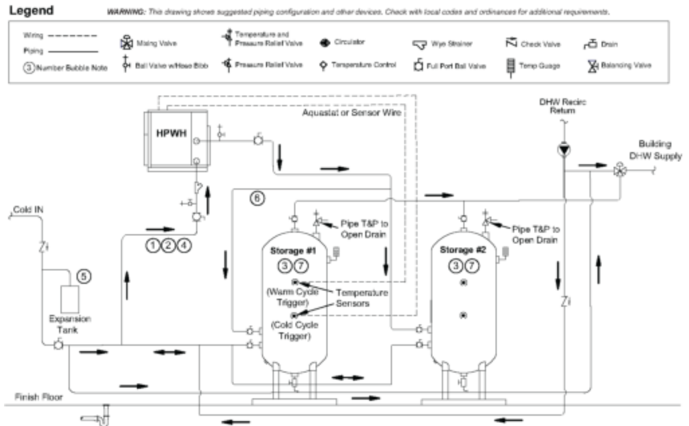
Figure 13. Multi-pass piping concept
