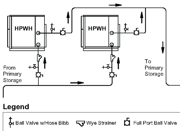
Figure 11. Piping considerations
