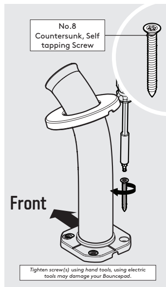
B5 Secure the Static60 to the surface with the 4x countersunk fixings.
