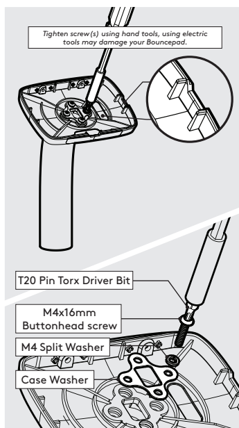
1 Locate & attach the Shell to the Static 60 in the correct orientation.
