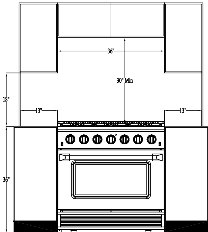
Installation Diagram
