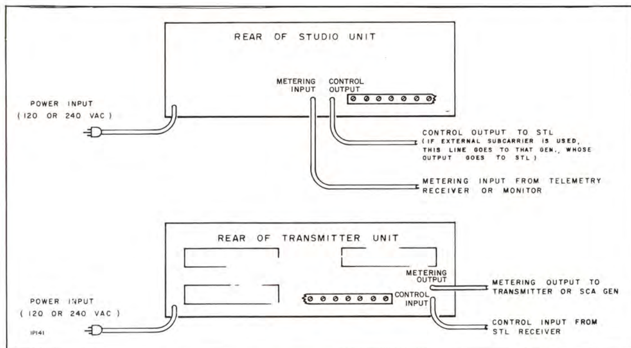
Figure 13. Wireline Interconnections
