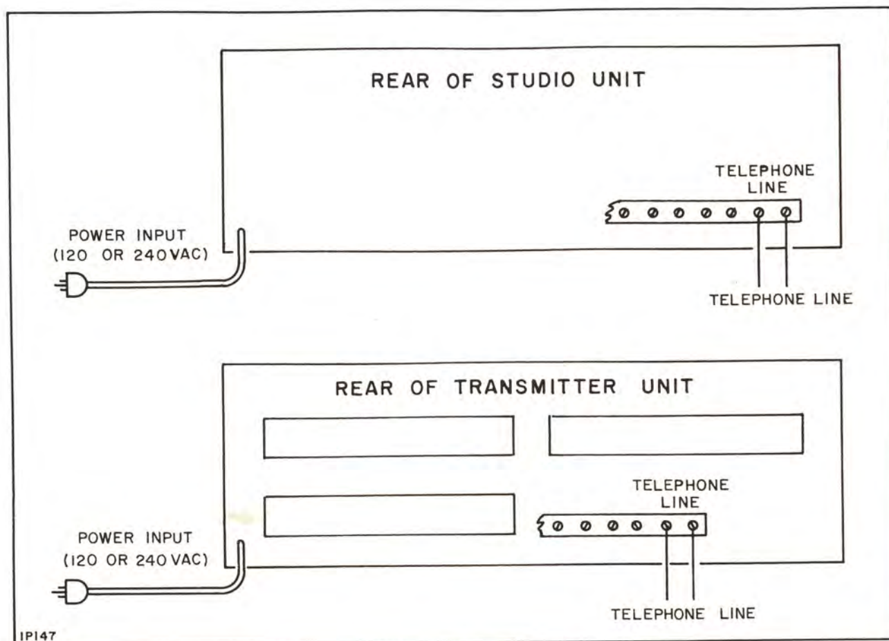
Figure 12. Telephone Line Interconnections
