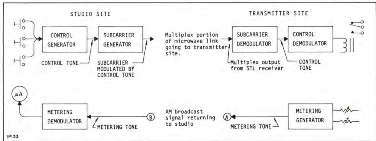
Figure 3. Basic BTR-15BR Wireless AM Remote Control System
