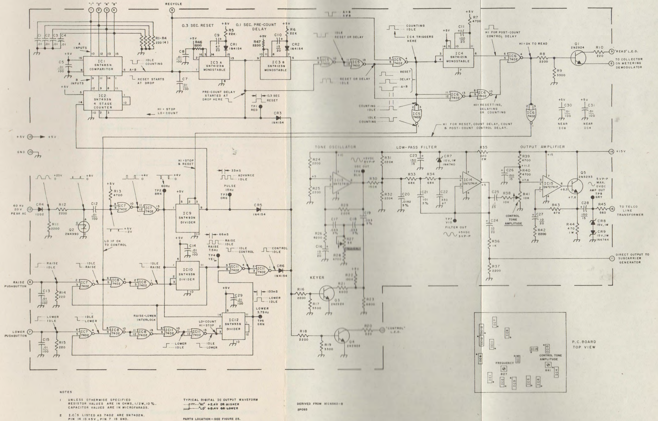
Figure 40. Control Generator, Schematic Diagram
