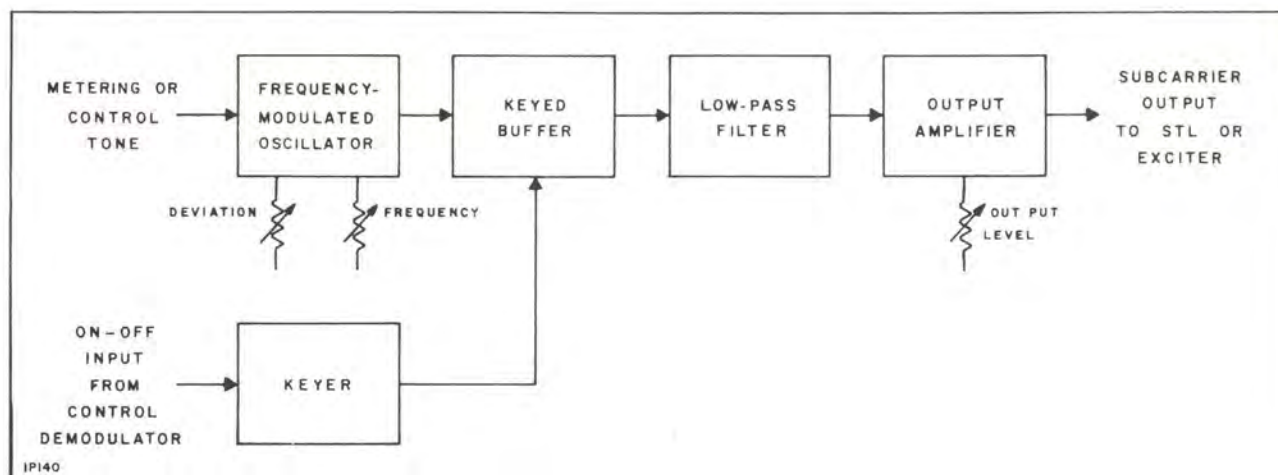
Figure 5. Subcarrier Generator, Block Diagram
