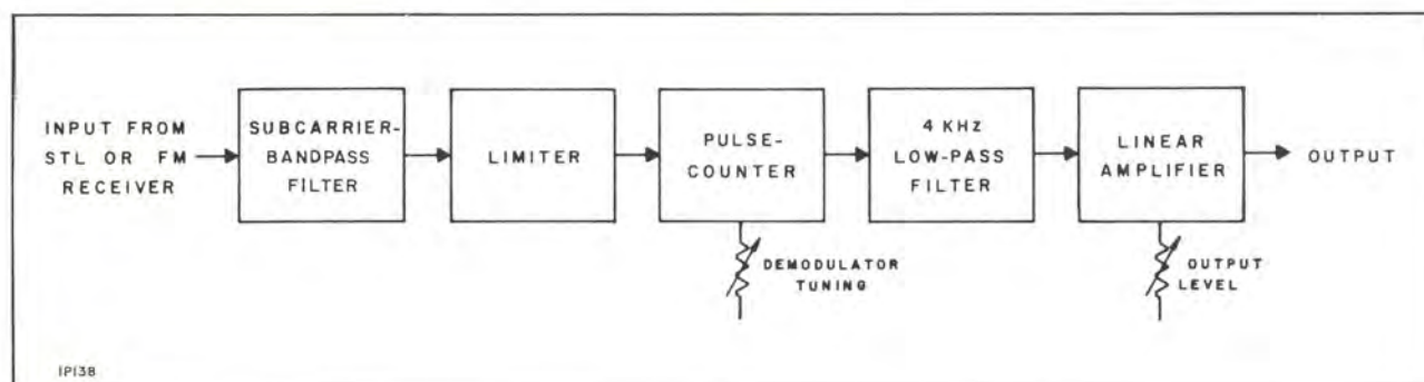
Figure 6. Subcarrier Demodulator, Block Diagram
