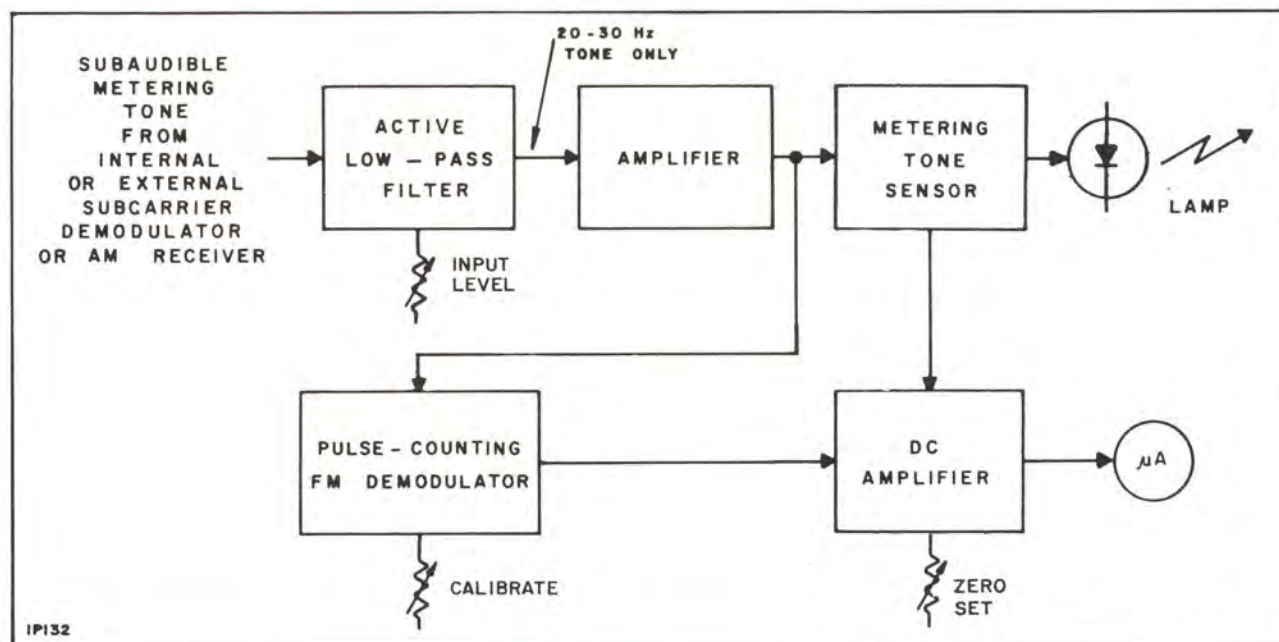
Figure 8. Subaudible Metering Demodulator, Block Diagram.
