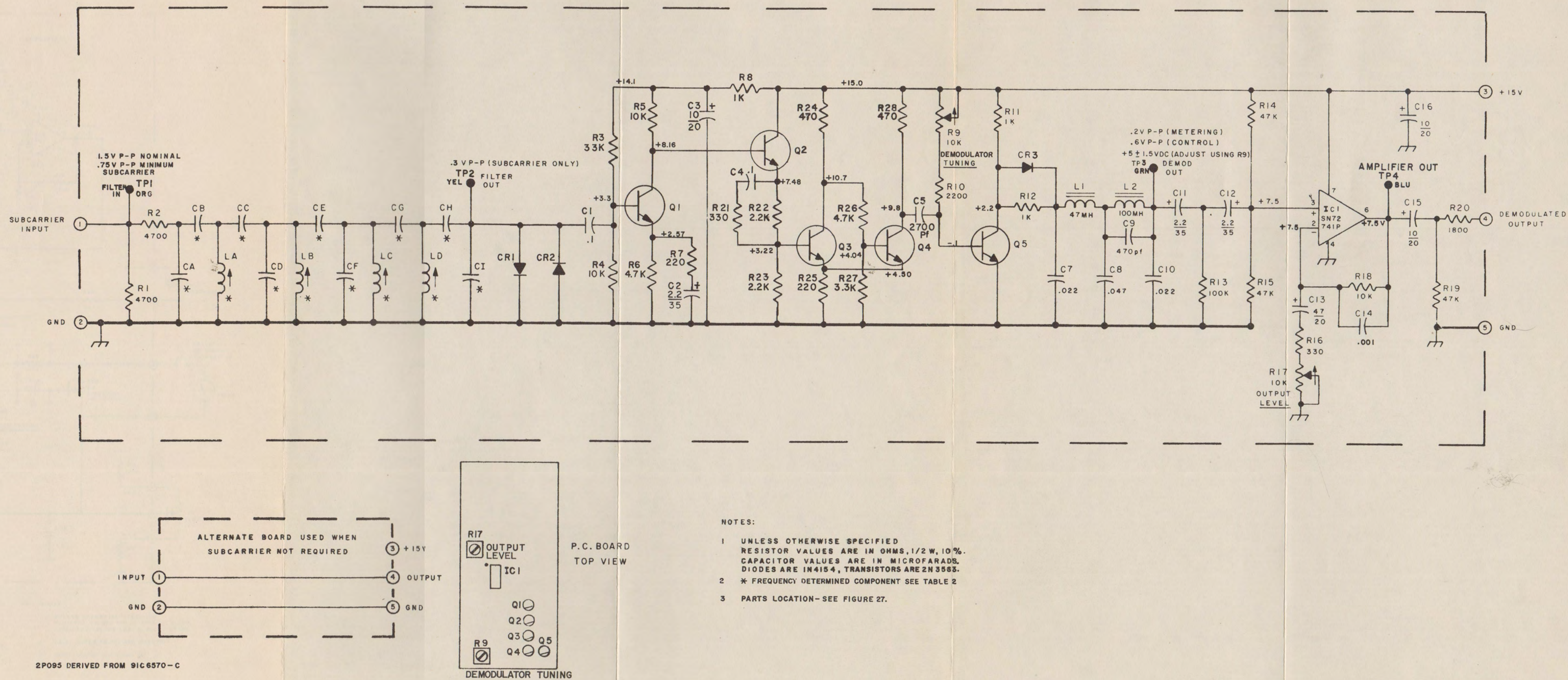
Figure 42. Subcarrier Demodulator, Schematic Diagram
