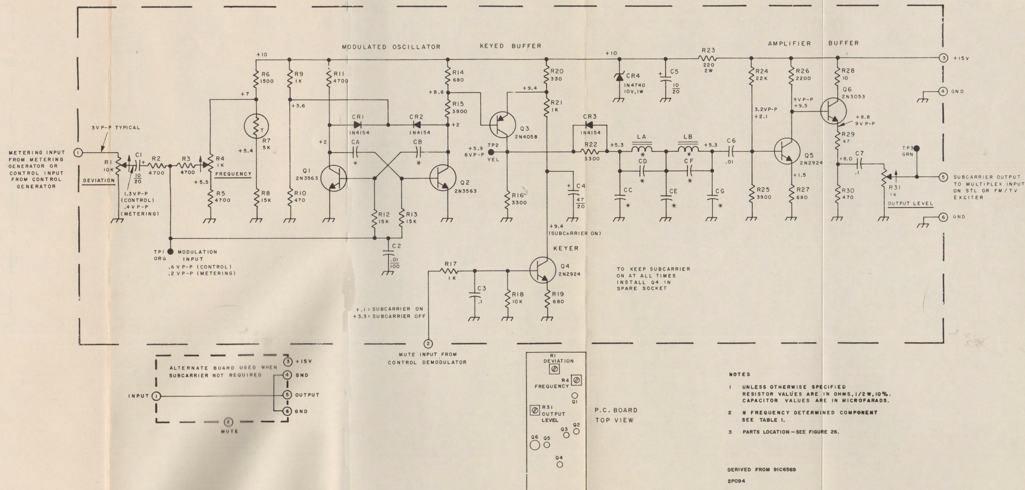
Figure 41. Subcarrier Generator, Schematic Diagram
