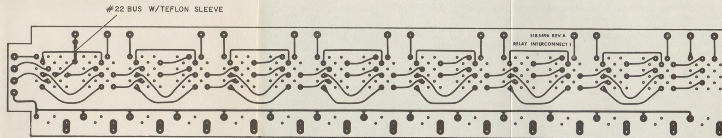
RELAY INTERCONNECT 1
