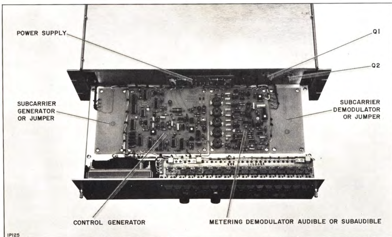
Figure 18. Studio Unit, Front View, Drawer Open
