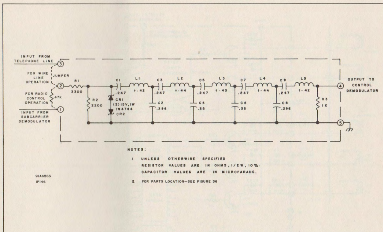
Figure 46. Control Bandpass Filter, Schematic Diagram
