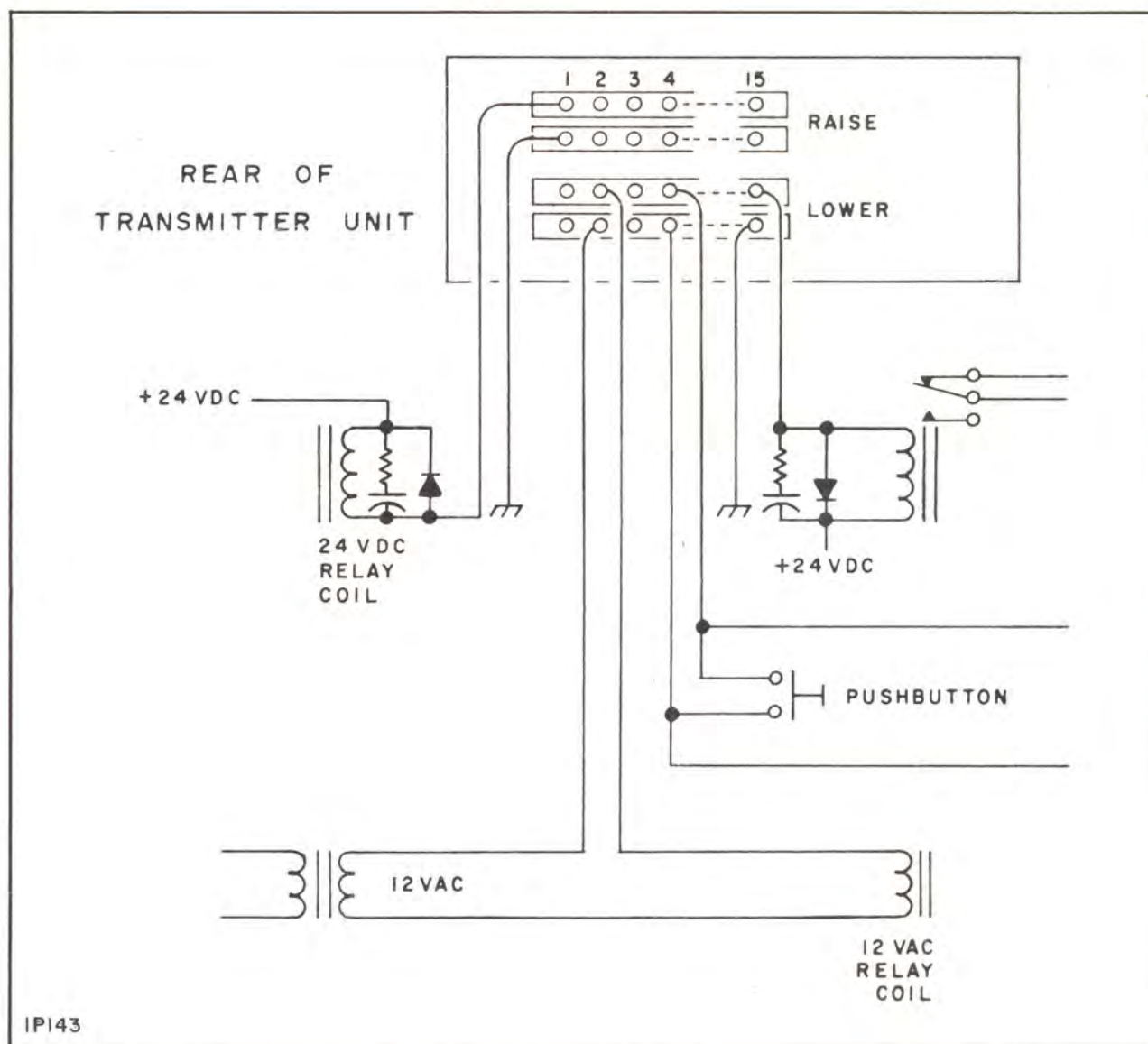
Figure 16. Control Circuitry, Simplified Schematic
