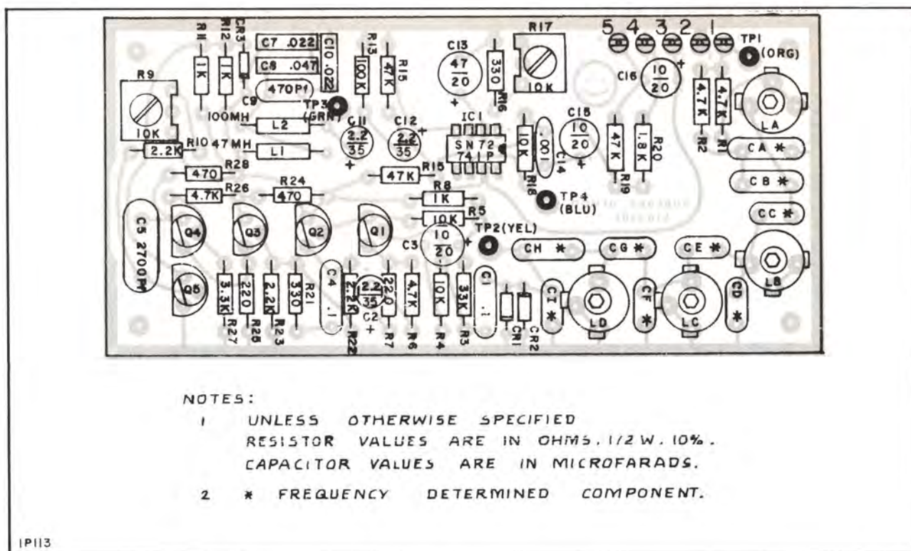
Figure 27. SU and TU Subcarrier Demodulator, Parts Location
