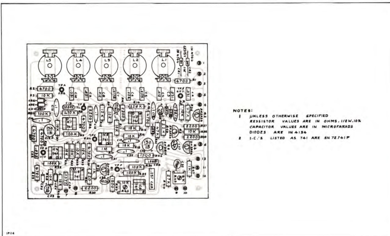
Figure 28. SU Audible Metering Demodulator, Parts Location
