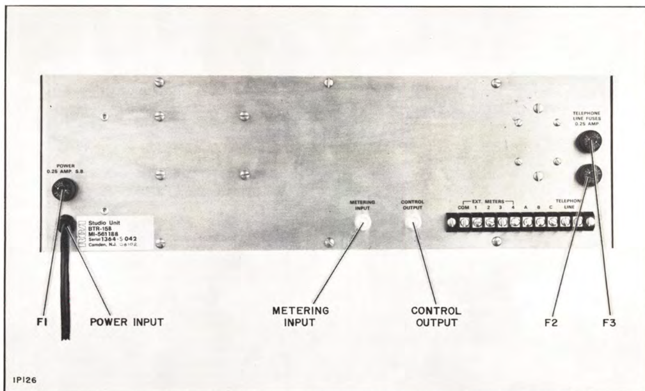
Figure 19. Studio Unit, Rear View
