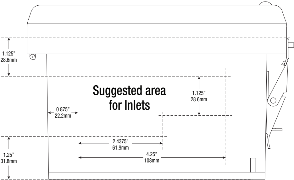
Fig. 2 - Bottom of enclosure
