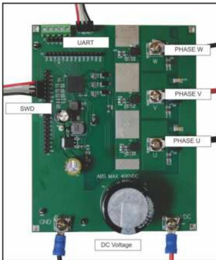
Figure 7: PAC5556AEVK2 Evaluation Module Connections
