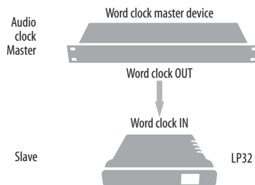
Figure 4-16: Slaving the LP32 to word clock. For the LP32 clock source, choose 'Word In'.
