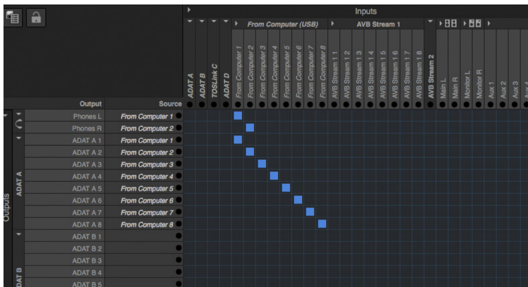
Figure 7-6: An example of routing computer channels (from host audio software) to the outputs on an LP32. Computer channels 1-2 are being split to two pairs of outputs: Phones L-R and ADAT A 1-2.
