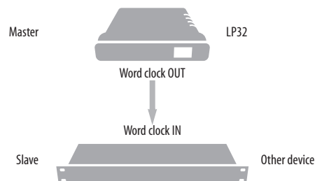
Figure 4-15: Slaving another digital audio device to the LP32 via word clock. For the LP32 clock source, choose any source besides word clock, as it is not advisable to chain word clock.
