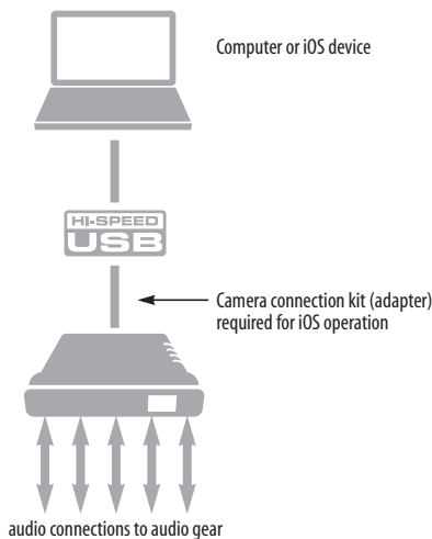
Figure 5-1: Using the LP32 as an audio interface.
