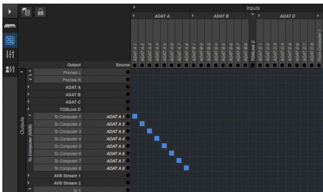
Figure 7-7: An example of routing physical inputs on the LP32 to computer channels (for host audio software).
