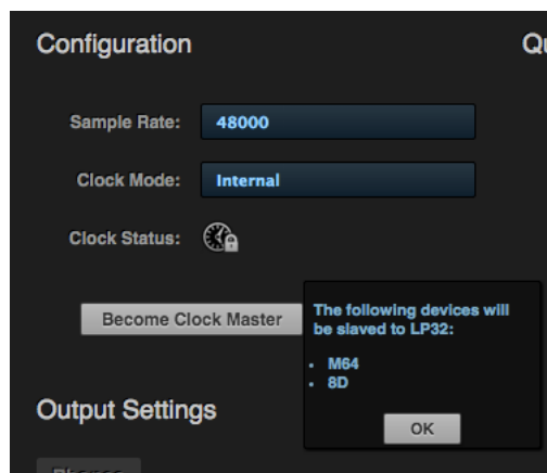
Figure 4-17: Choosing a clock master.
