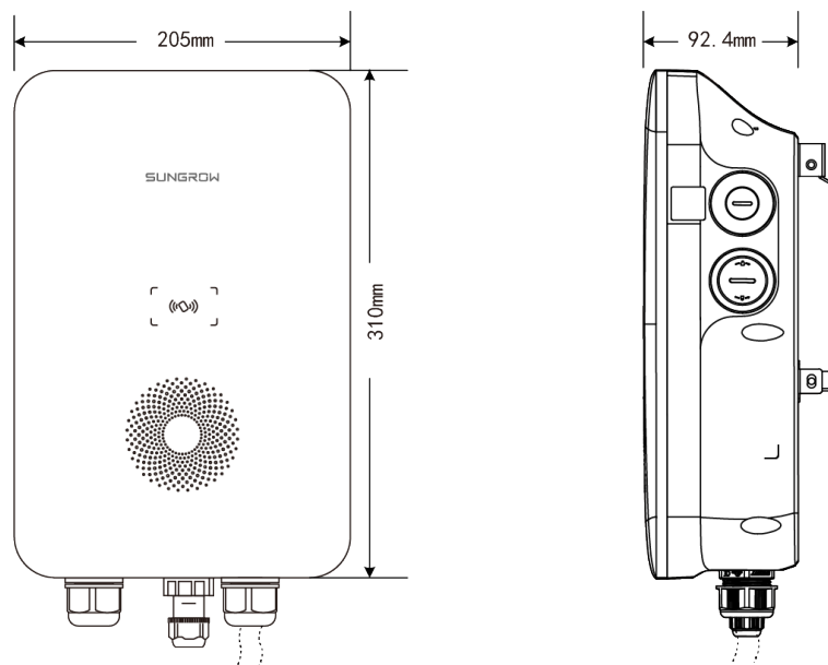
figure 2-1 Appearance and dimensions
