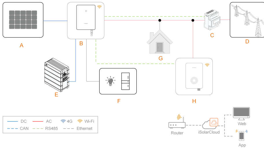
figure 2-4 System topology diagram of the solar-storage-charging solution
