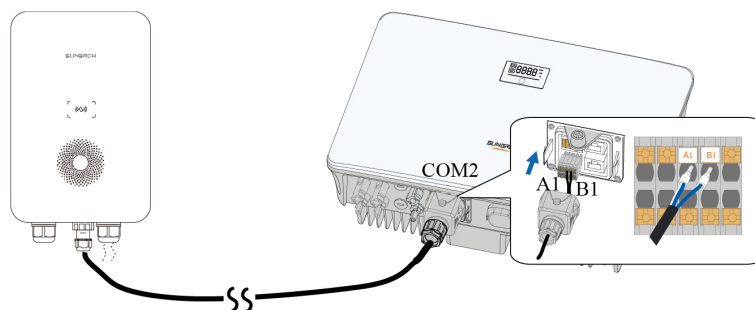
figure 3-5 Connect to an inverter(SHRS)
