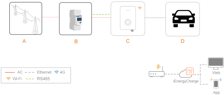
figure 2-3 System topology diagram of EV charger
