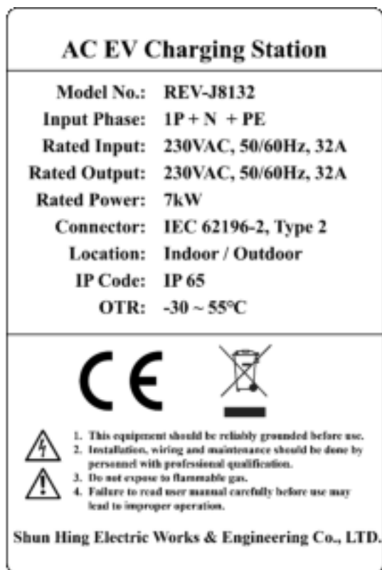
Fig. 4-4 The location and content of the nameplate
