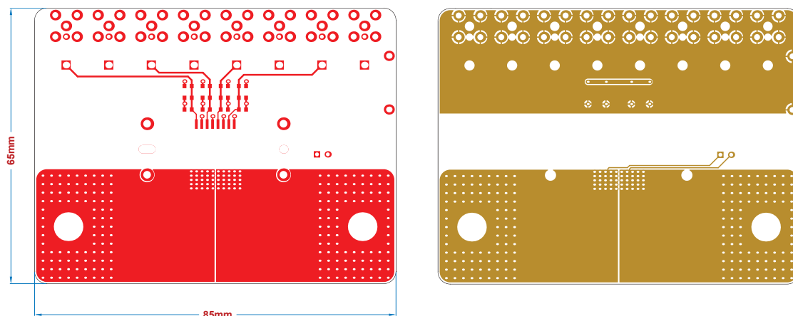
Figure 8: MC Generic Evaluation Board Top Layer (left) and Interior Layer 1
