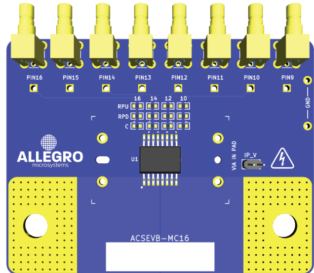
Figure 1: MC Evaluation Board
