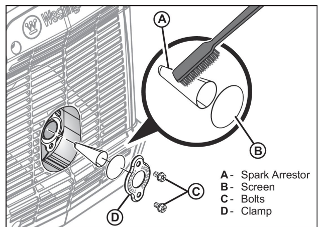
Figure 33 Remove and Clean the Spark Arrestor
