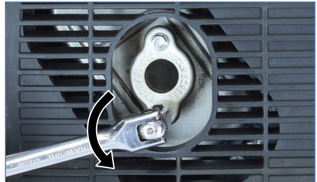
Figure 32 Remove the Spark Arrestor Clamp
