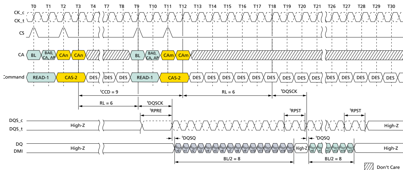
Figure 112: Consecutive READ: t_{CCD} = \text{MIN} + 1 , Preamble = Static, 1.5n\text{CK} Postamble
