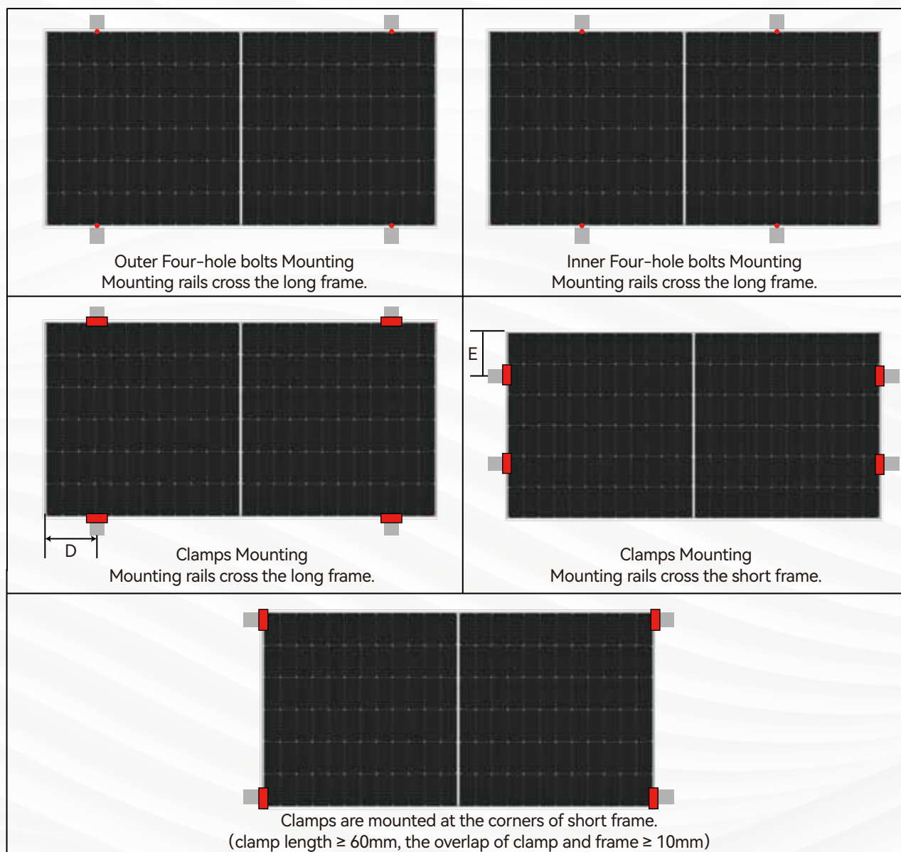
Figure 7 Mono-facial Module Installation Position
