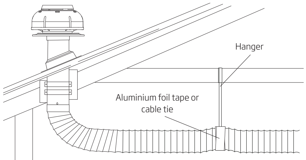
Figure 9 Examples of securing ducting
