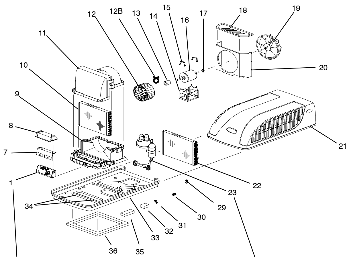
ITEM 23 - COMPRESSOR ASSEMBLY
