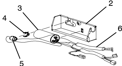
ITEM 1 - CONTROL BOX ASSEMBLY
