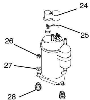
ITEM 23 - COMPRESSOR ASSEMBLY
