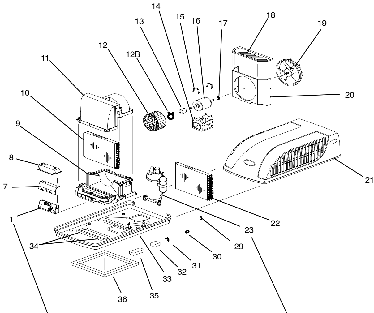
ITEM 23 - COMPRESSOR ASSEMBLY
