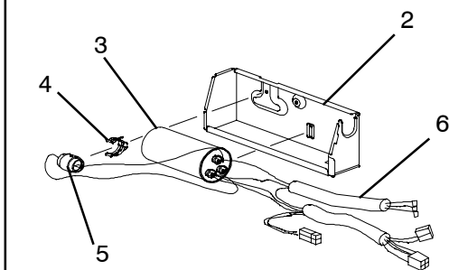
ITEM 1 - CONTROL BOX ASSEMBLY
