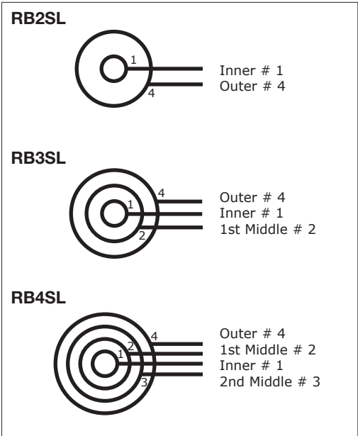
Gas valve and burner ring matching.
