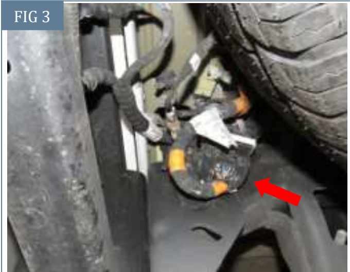
(Fig 3) Locate and remove wiring harnesses leading to bumper
