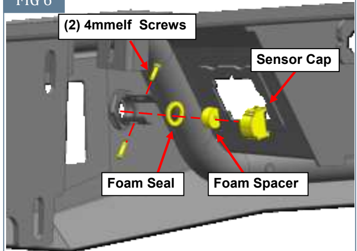
(Fig 6) Insert sensor assembly into the sensor mount on back of Bumper. Use 4mm Screws to lock sensor in place.
