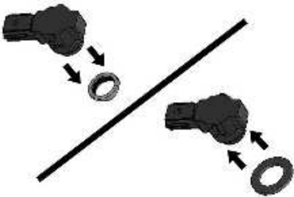
(Fig 5) Remove original silicone seal from sensor. Slide included Foam Seal over end of sensor
