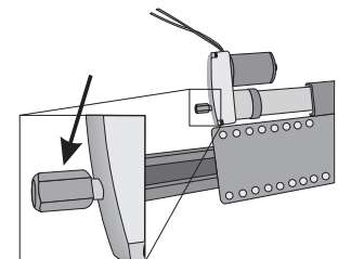
Fig. 8.6 Main slide hex head
