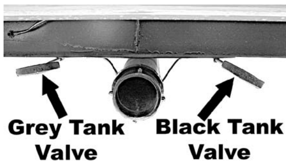
Fig. 7.7 Black & Grey tank dump valves
