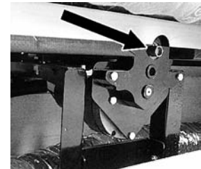
Fig. 9.4 RBW slide hex head
