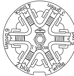
Fig. 4.2 7-way trailer plug Car end, rear view
