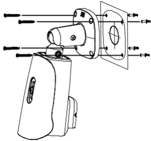
Figure 3-1 Installing bracket
