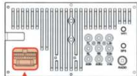
Power/Speaker/SWC Harness
