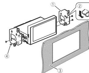
① Factory radio-mounting bracket ② If the pawl interferes with installation, you may bend it down out of the way. ③ Dashboard or console ④ Flush surface screw Be sure to use the screws supplied with this product.
