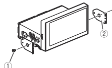
① Screw for fixing the side bracket ② Side bracket
