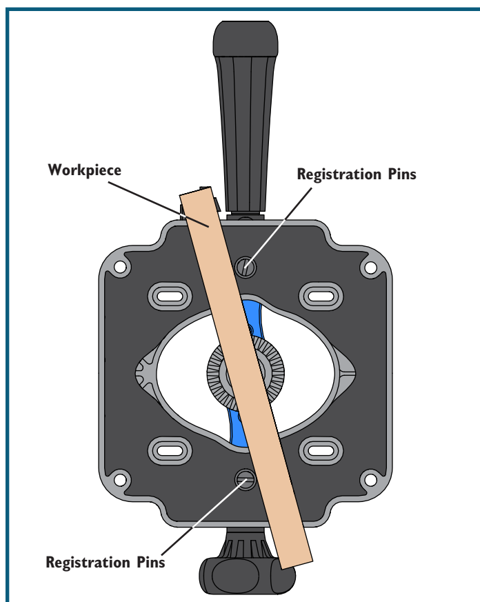
Fig. 3 - Bottom View
